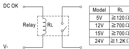
(c) Relay
